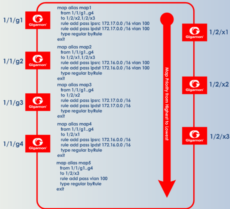
Figure 1: Sending Subnets and VLANs to Different Ports
