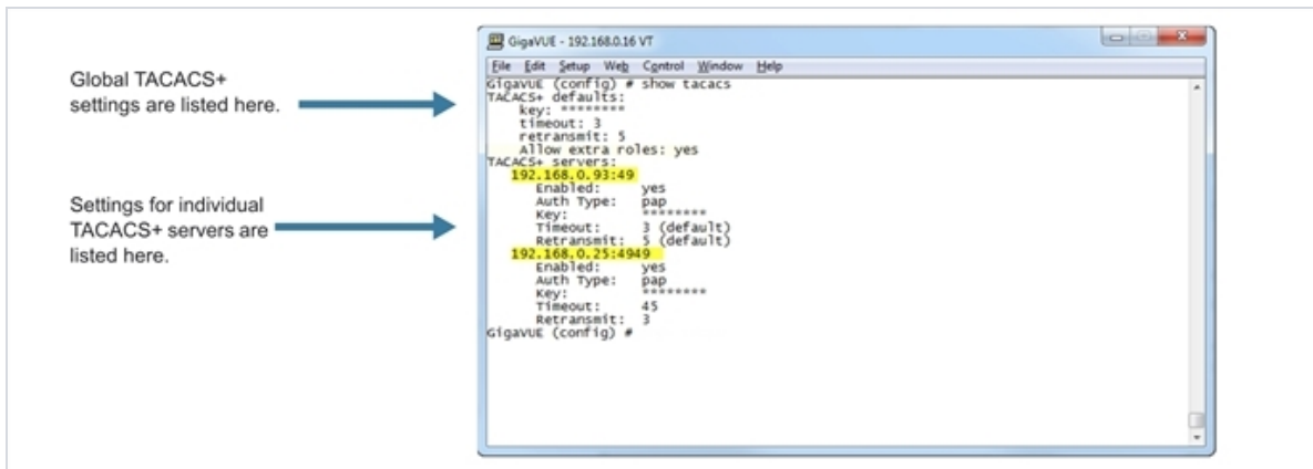
Figure 2: Results of show tacacs Command
