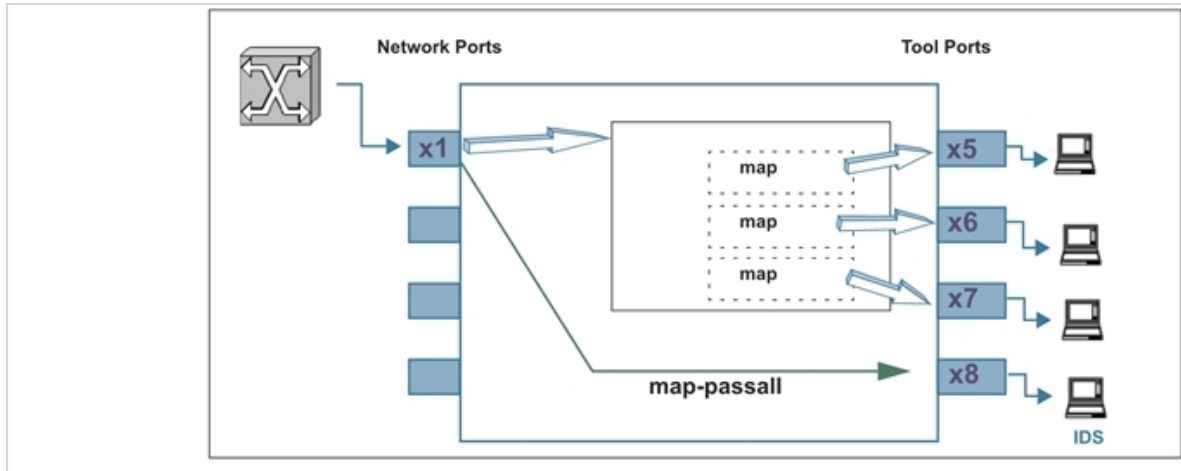
Figure 1: Sending All Traffic to IDS
