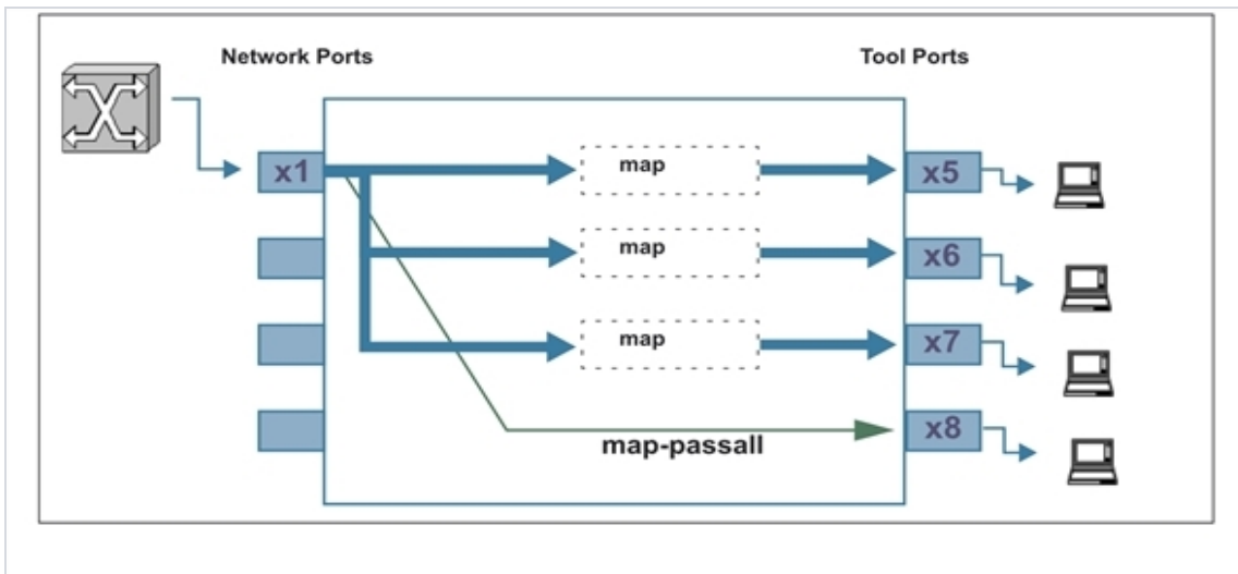
Figure 3: Adding a Map-passall for Temporary Troubleshooting
