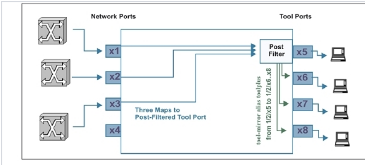
Figure 5: Adding tool-mirrors to Multiple Tool Ports
