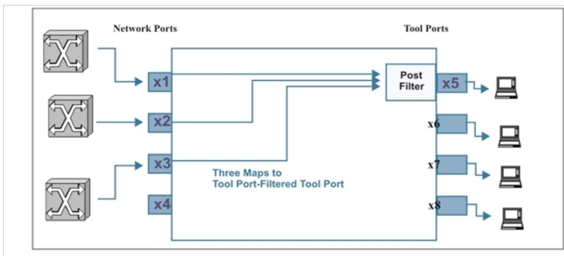
Figure 4: Creating a Tool-mirror
