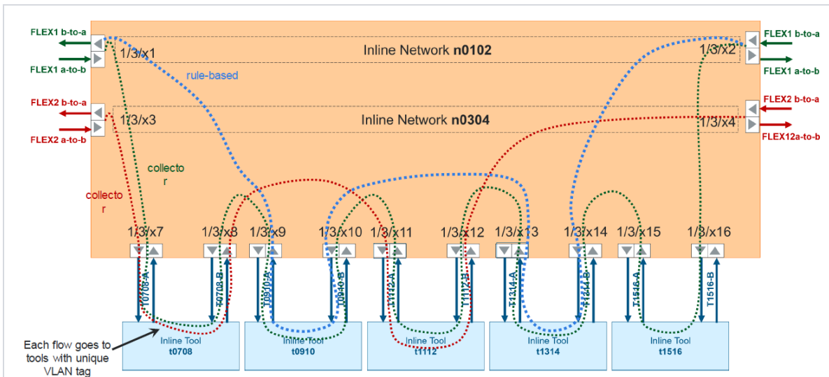
Figure 1: Example 4 Inline Tool Sharing by Multiple Inline Flows
