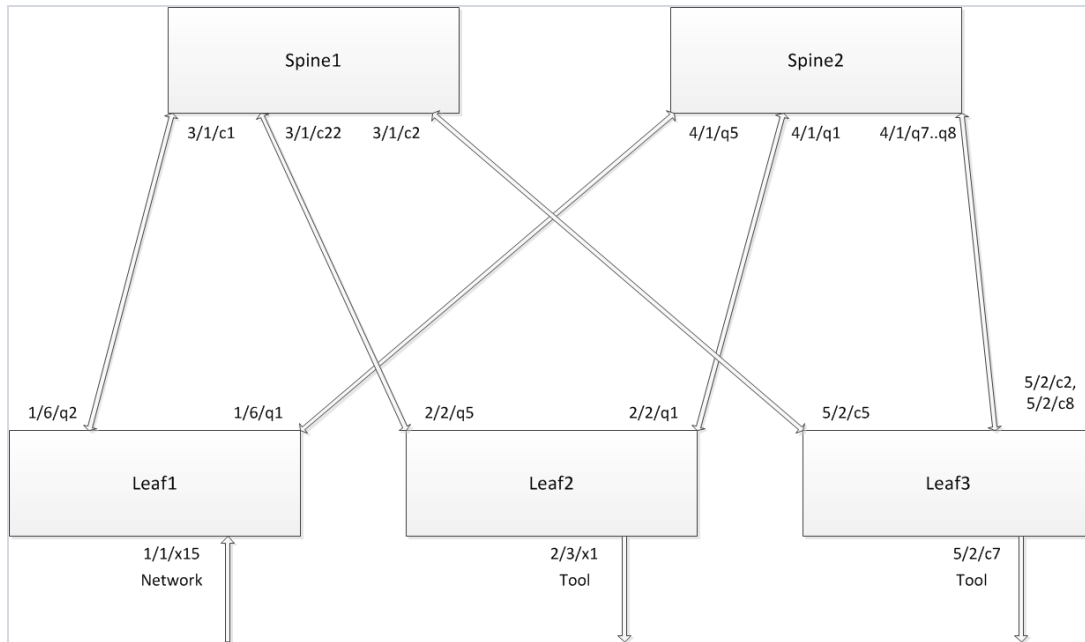
Figure 1: Configuration Leaf Spine Topology
