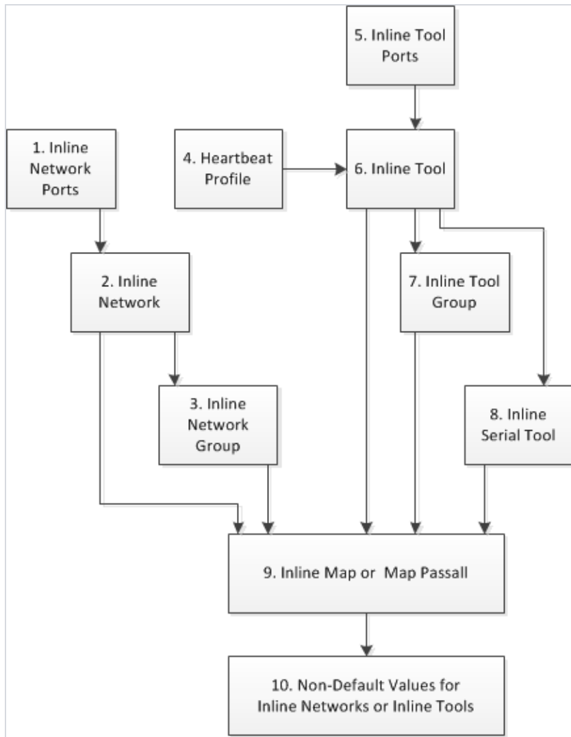
Figure 1: Configuration Steps for Inline Bypass Solutions
