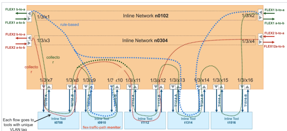
Figure 1: Example 6 Inline Tool Sharing by Multiple Inline Flows
