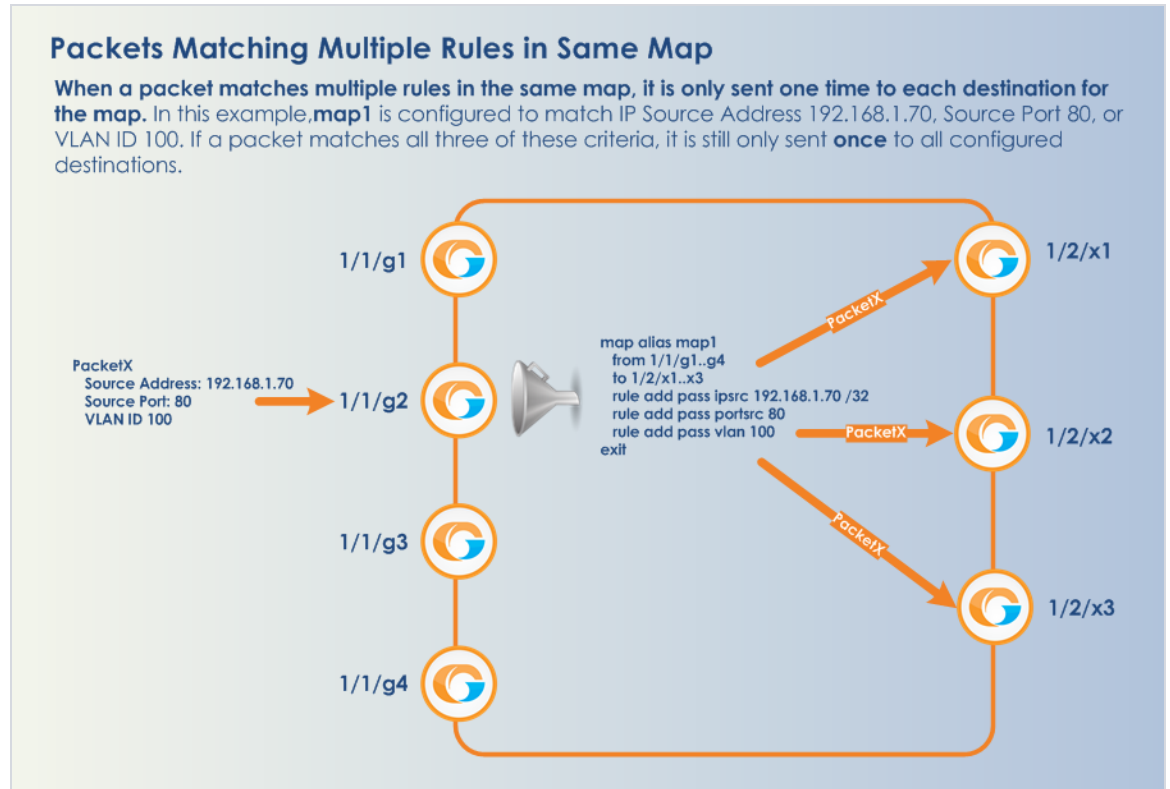
Figure 1: Packet Matching Multiple Rules in Same Map
