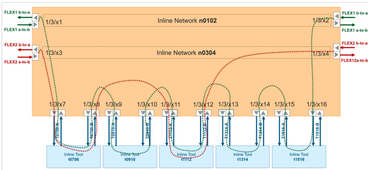
Figure 1: Example 2 Inline Tool Sharing by Multiple Inline Flows
