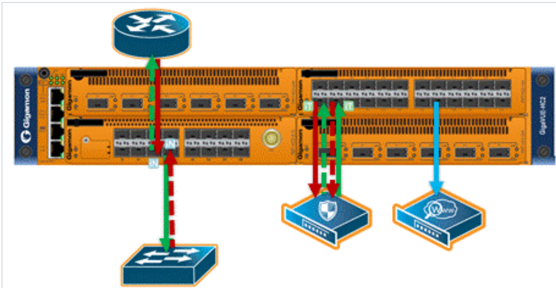
Figure 1: Logical Bypass
