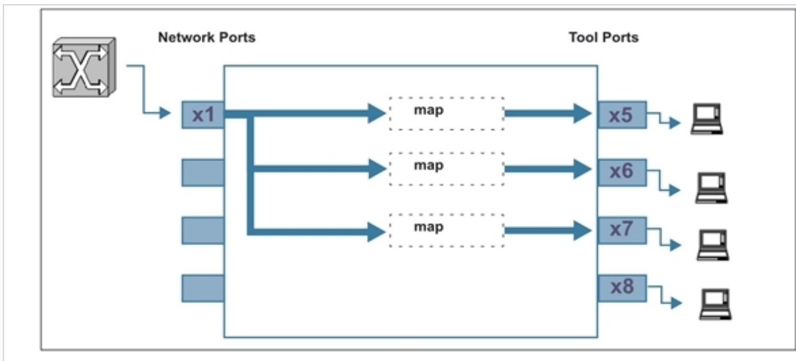
Figure 2: Existing Map on Network Port 1/2/x1
