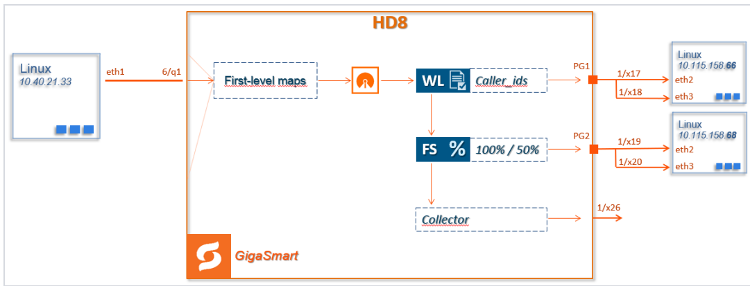
Figure 1: SIP/RTP Load Balancing Topology
